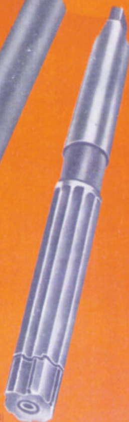
CARBIDE TIPPED REPLACEABLE HEAD MACHINE REAMERS
